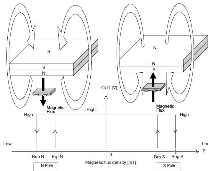
Fig 4, Magnetic Operation Characteristic of AS1833AOD
