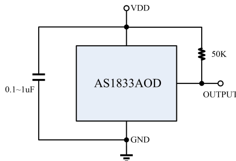
Figure 1, Typical Application Circuit of AS1833AOD
