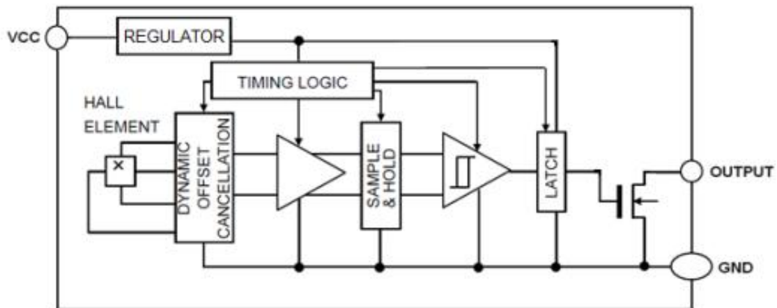
Figure2, Block Diagram of AS1833AOD
